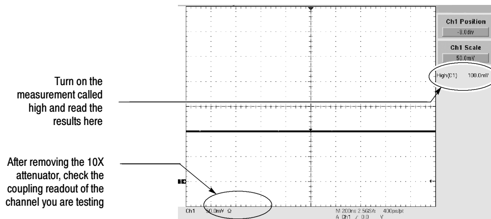
Figure 4-8: Check of maximum input voltage
