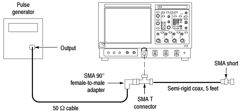
Figure 4-18: Delta time accuracy test hookup for TDS6000B Series
